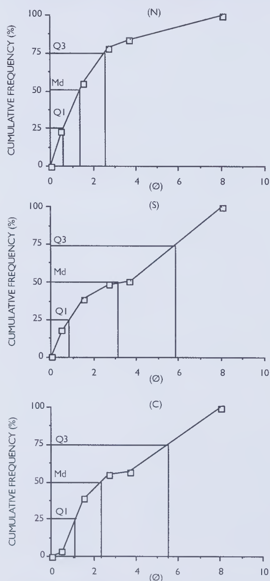
Figure 3. Cumulative weight frequency and particle diameter ( \phi ) for sediments from Collie River Site 11, north (N); south (S); and centre (C). \phi = -\log_2 (particle size mm).
